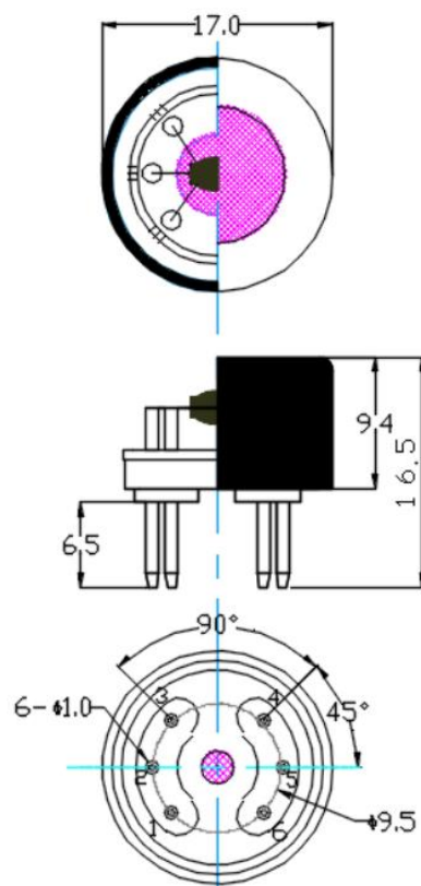
Fig1. Sensor Structure
