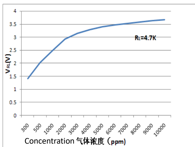
Fig5.Sensitivity Curve
