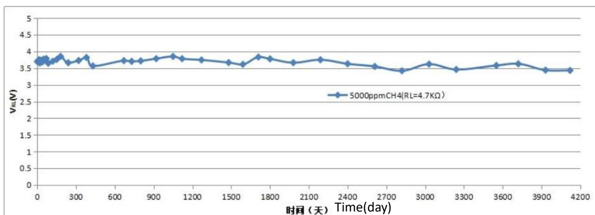
Fig7.long-term Stability
