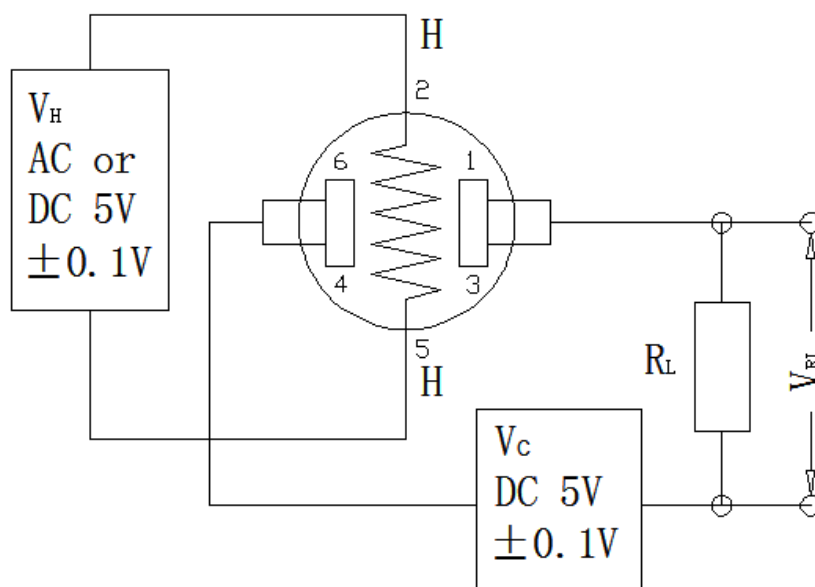
Fig2. MQ-4B Test Circuit
