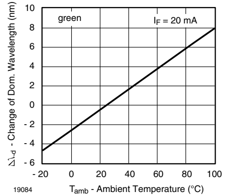
Fig. 12 - Change of Dominant Wavelength vs. Ambient Temperature
