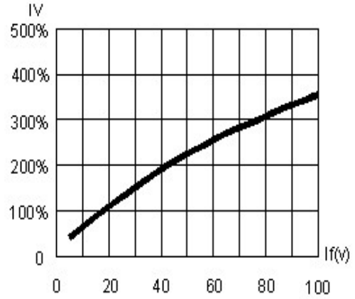
Fig.2 Relative Luminous Intensity vs Forward Voltage
