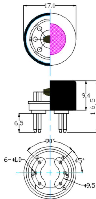
Fig1. Sensor Structure
