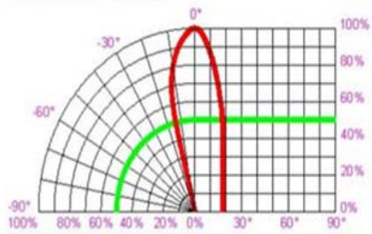
Fig.6 Relative Luminous Intensity vs viewing angle
