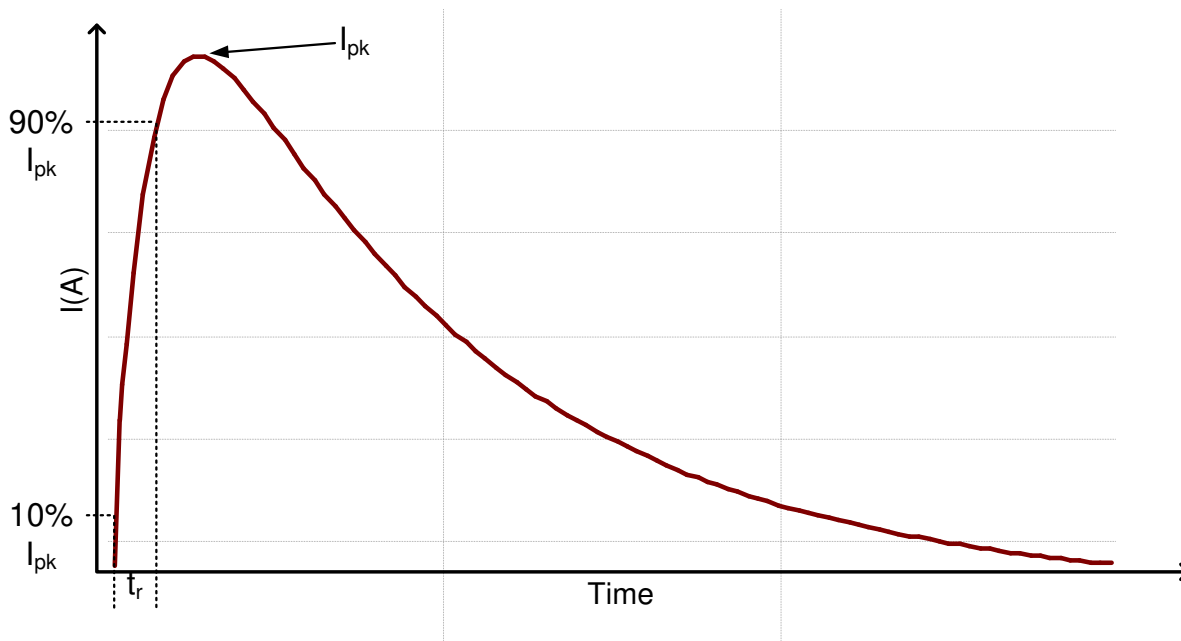
Figure 10-2. HBM Curve
