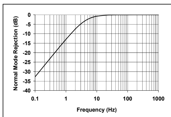
FIGURE 4-4: HPF Magnitude Response ( MCLK = 3.58 MHz).
